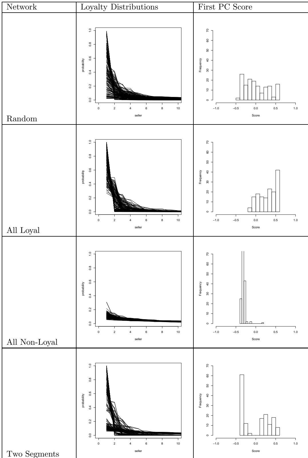
Figure 10: Simulated Loyalty: The middle column shows the observed bidder loyalty distributions; the right column shows the first functional principal components score.
