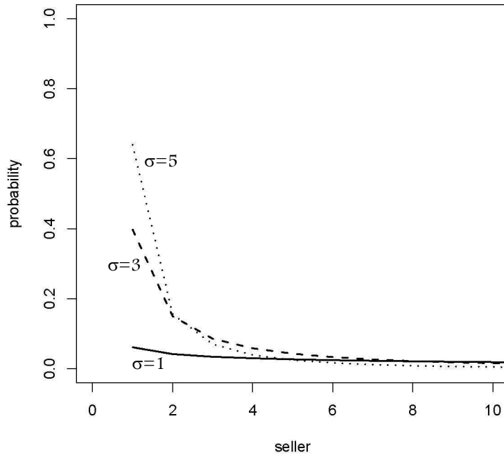
Figure 9: Simulated e-Loyalty: Larger values of \sigma correspond to higher levels of loyalty to the same seller.
