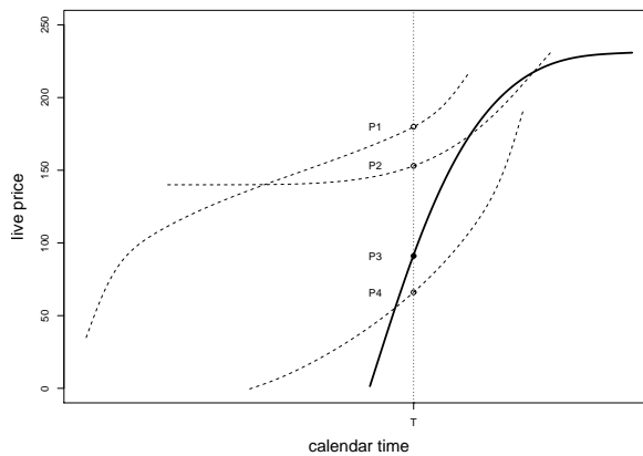
Figure 5: The solid line is the focal auction and the broken lines correspond to simultaneous, competing auctions. T corresponds to the time of decision making and p_1 through p_4 is the price information from all auctions available at that time.
