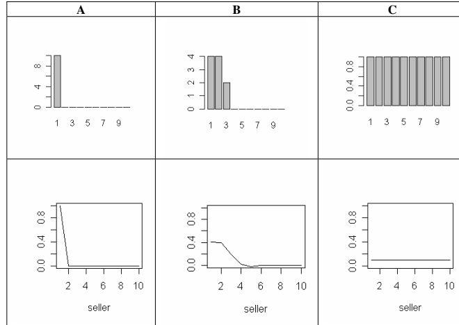
Figure 8: Illustration: The top panel shows the observed loyalty distribution for each bidder from Figure 7; the bottom panel shows a smooth representation of the standardized distribution using smoothing splines.
