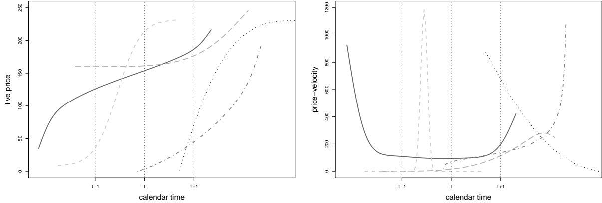
Figure 4: Smooth price paths (left panel) and corresponding velocities (right panel). The solid line corresponds to the focal auction; the broken line illustrate simultaneous, competing auctions.
