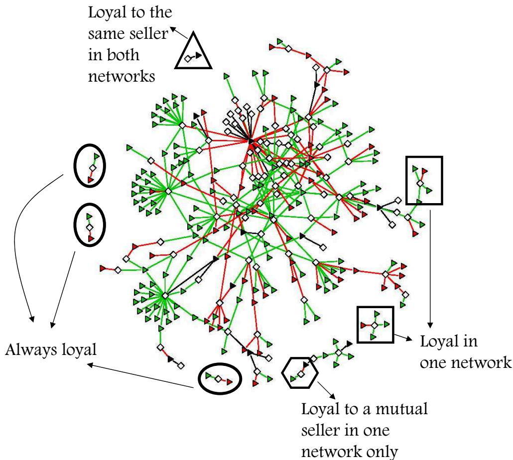
Figure 11: e-Loyalty networks for Parker and Cross pens. Sellers are denoted by triangles, bidders by squares; arcs denote an interaction between the two. Red (green) arcs denote bidder-seller interactions exclusively for Parker ( Cross ) pens, black arcs denote an interaction between a bidder and a seller for both brands.
