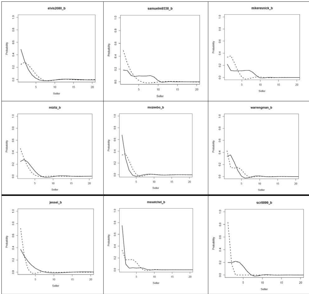
Figure 13: Comparison of bidders' loyalty curves in different product-networks. The solid lines correspond to loyalty in the Cross network, the dashed lines correspond to the Parker -loyalty.
