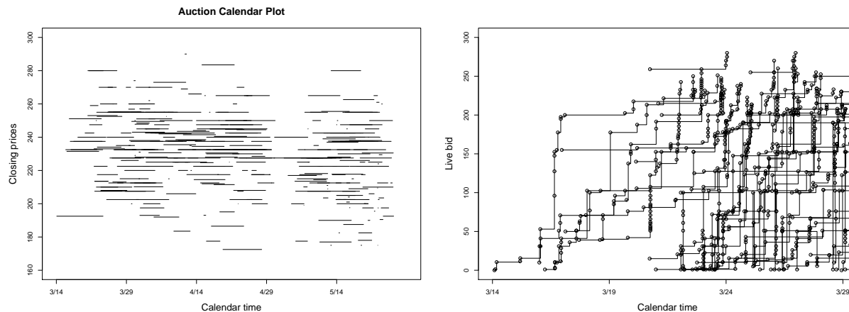
Figure 3: Left panel: Calendar plot of closing prices vs calendar time. Each line in the graph represents an auction, the length of the line corresponds to the length of the auction; the y-axis denotes the closing price, and the x-axis denotes calendar time. Right panel: A snapshot of the live price process of competing products during eBay auctions. The circles denote the arrival of new bids. The horizontal lines mark the time periods during which the price in an auction remains unchanged.
