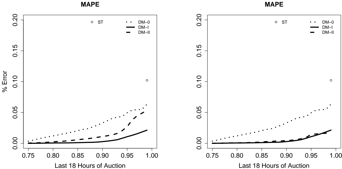
Figure 2: Left panel: Models DM-I, DM-II, ST and DM-0 without bidder competition components; Right panel: same models with the bidder competition.
