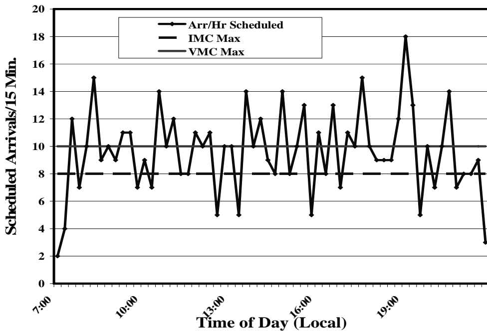
Figure 3. LGA Scheduled Number of Arrivals in 15 minute increments compared to the FAA estimate of safe aircraft operational separation of 8 (32 Arrivals / Hr.) under Instrument Meteorological Conditions (IMC) (FAA 2001)
