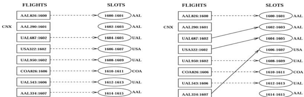
Figure 7: Execution of Compression Algorithm
