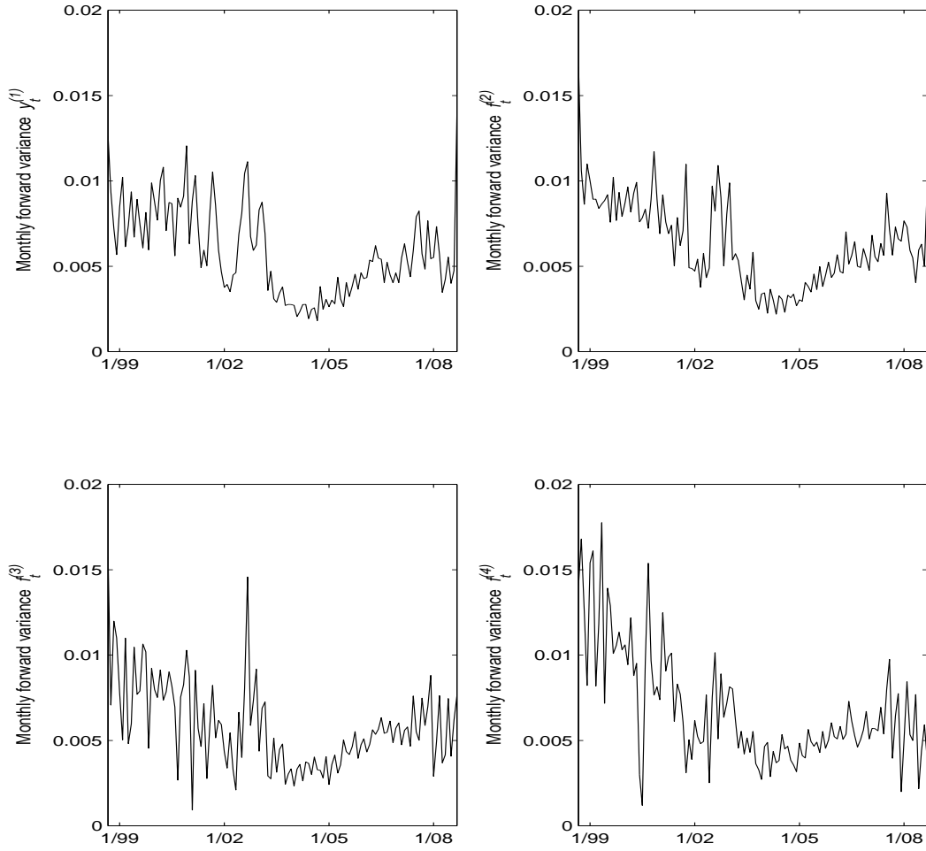
Fig. 1. Time series behavior of forward variances
