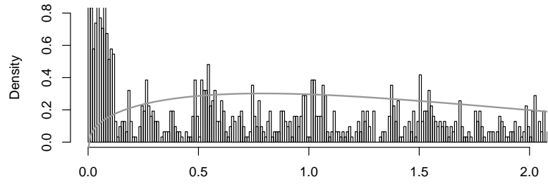
k=25 Transform
