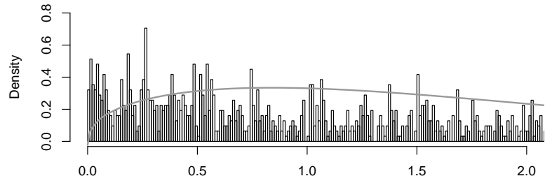
k=8 Transform
