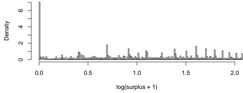
k=25 Transform
