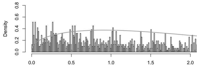
k=4 Transform
