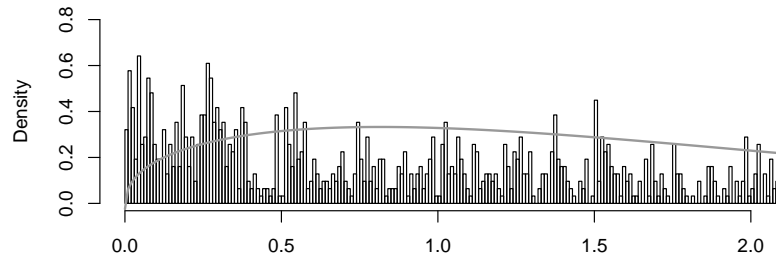
k=10 Transform
