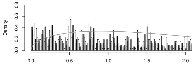
k=5 Transform
