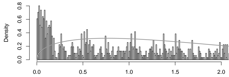
k=20 Transform
