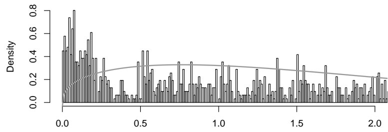
k=16 Transform
