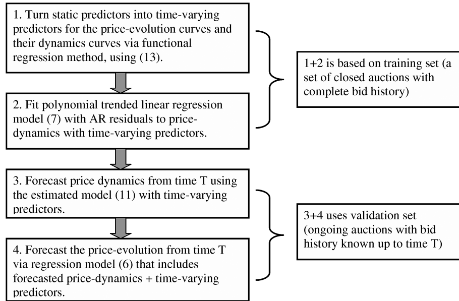
Figure 9. Flowchart of Dynamic Forecasting Model.
