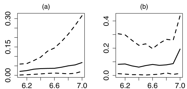
Figure 14. Mean Absolute Percentage Errors (MAPEs). MAPE_1 (a) is the error between the forecasted price curve and the true functional price curve; MAPE_2 (b) is the error between the forecasted price curve and the actual current auction price. The dotted lines correspond to the 5th and 95th percentiles.
