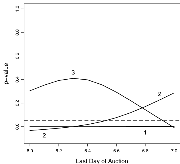
Figure 10. p -Value Curves for x_1, x_2 , and x_3 Over the Last Auction Day. Consistent with the three predictors, we denote 1 = opening bid, 2 = item value, and 3 = jump bidding. The dotted horizontal line marks the 5% significance level.
