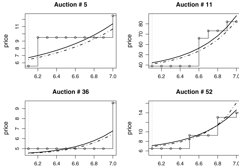
Figure 13. Dynamic Forecasting Results of Last-Day Price for Four Sample Auctions (—○— current auction price; — functional price curve; - - - forecast price curve).
