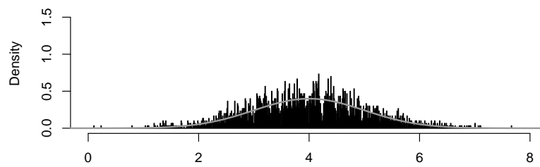
Local Regeneration Transform (k=5)
