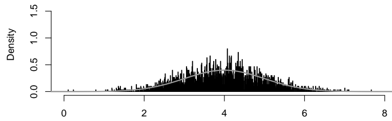
Local Regeneration Transform (k=10)
