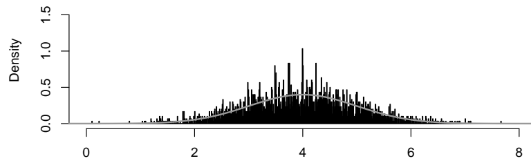
Jitter Transform (Uniform, delta=0.01)
