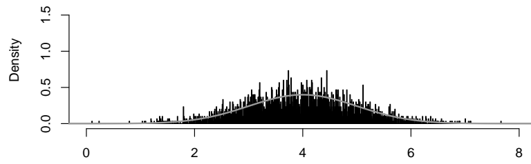
Unobservable Normal Sample
