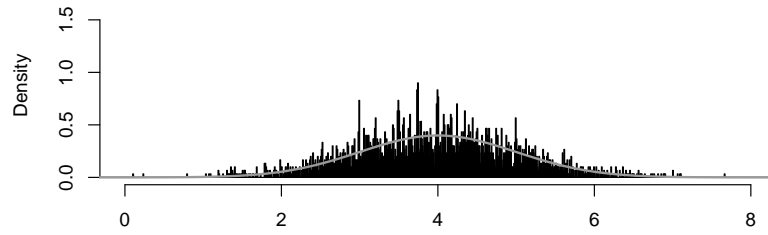
Jitter Transform (Normal, delta=0.02)
