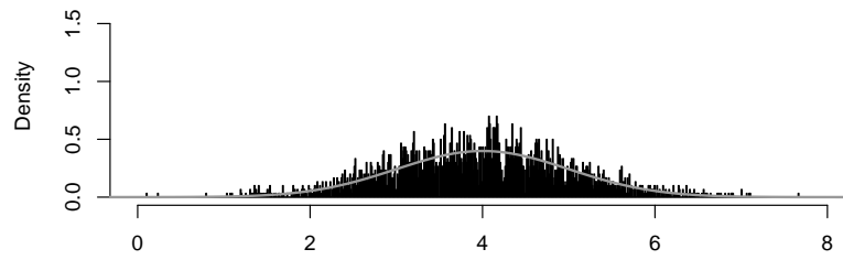
Local Regeneration Transform (k=8)
