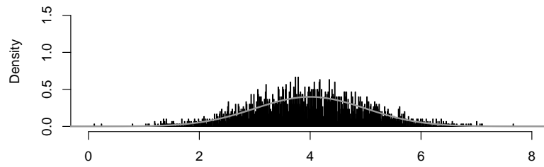
Jitter Transform (Normal, delta=0.12)
