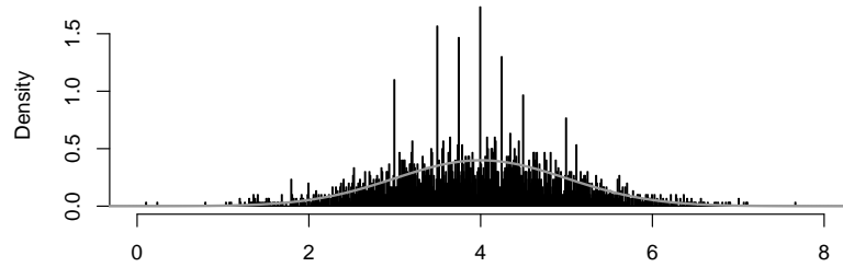
Contaminated Normal Sample
