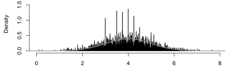
Jitter Transform (Normal, delta=0.01)
