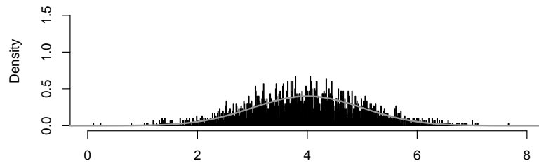
Jitter Transform (Uniform, delta=0.07)
