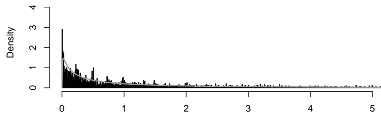
Jitter Transform (Normal, delta=0.07)
