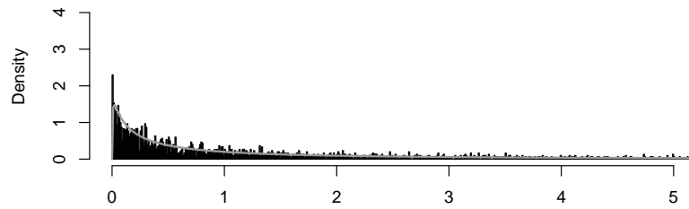
Jitter Transform (Uniform, delta=0.07)
