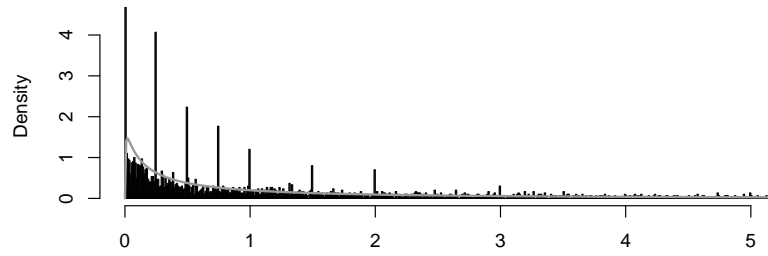
Contaminated Lognormal Sample
