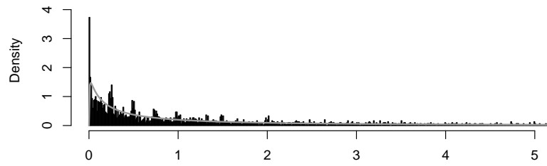
Jitter Transform (Normal, delta=0.05)
