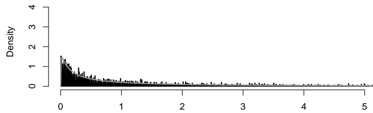
Jitter Transform (Uniform, delta=0.12)
