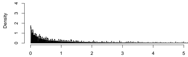
Jitter Transform (Uniform, delta=0.10)
