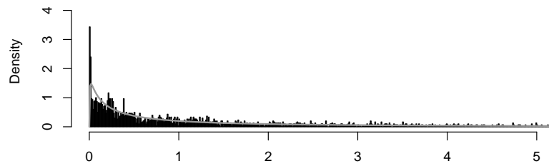
Local Regeneration Transform (k=20)
