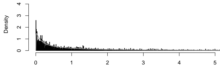
Local Regeneration Transform (k=10)
