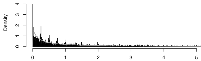
Jitter Transform (Uniform, delta=0.02)
