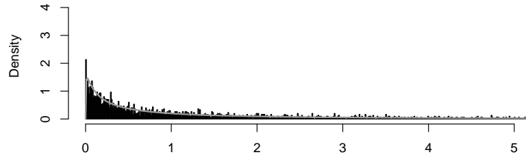
Unobservable Lognormal Sample
