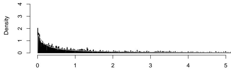
Local Regeneration Transform (k=8)
