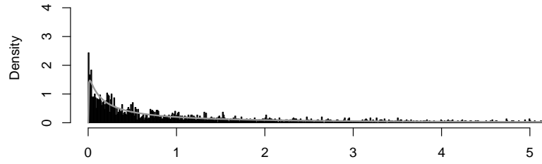
Jitter Transform (Uniform, delta=0.05)
