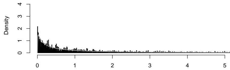
Jitter Transform (Normal, delta=0.12)
