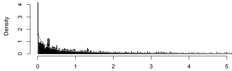
Local Regeneration Transform (k=25)
