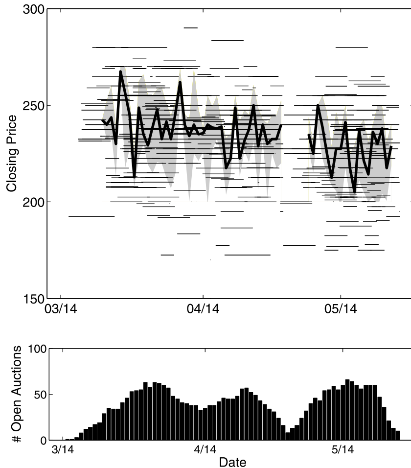
Figure 10. Auction calendar for 476 Palm M515 PDA auctions. In the top graph, each auction is a line extending from the auction start to the auction end. The vertical axis is the closing price. The thick line is the median daily closing price, and the shaded area extends between the lower and upper quartiles. The bottom graph shows daily auction volume: the number of open/active Palm auctions in the database, by date.
