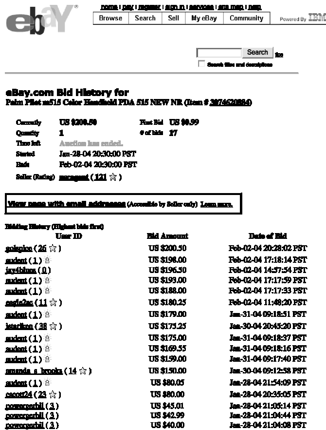
Figure 1. Bid History from eBay.com for closed auction of a Palm M515 PDA.
