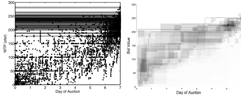
Figure 7. Profile plot (left) and shaded plot (right) for 158 seven-day Palm M515 auctions ( \alpha -transparency = .2)
