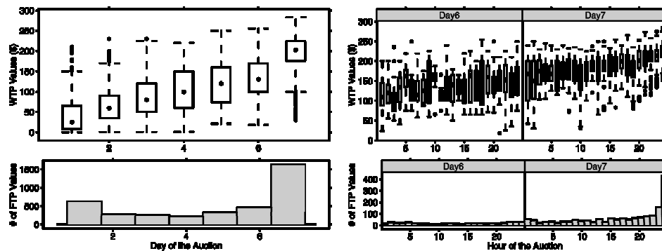
Figure 9. Daily (left) and hourly (for the last two days, right) WTP-value distribution and intensity over time for 158 Palm M515 PDA auctions.
