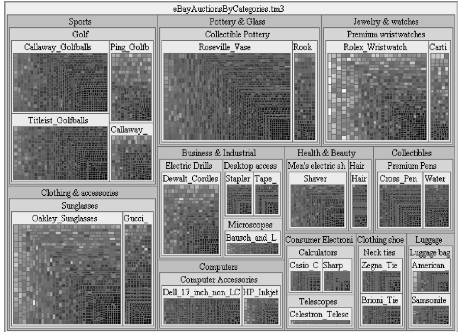
Figure 12. The eBay Auction Scene for 10,078 auctions. Grayscale represents number of bids per auction (black = low, white = high), size represents number of distinct bidders in auction
