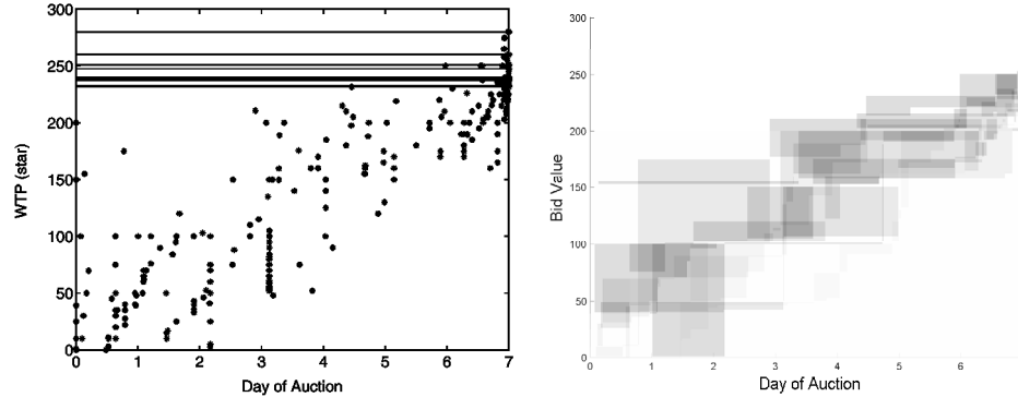
Figure 6. Profile plot (left) and shaded plot (right) for ten seven-day Palm M515 auctions ( \alpha -transparency = .2)
