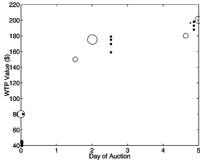
Figure 5. Profile plot for Palm M515 PDA, with circle size representing bidder feedback: Bigger circles represent higher feedback. The different colors represent distinct bidders (hollow circles are bids by single time bidders).
