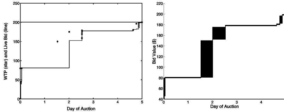
Figure 3. Profile plot and shaded plot for a single Palm M515 PDA five-day auction. Left panel: WTP values (stars) and live-bid values (step-function line) for a single auction. The horizontal line at $200.50 displays the closing price. Right panel: The area between the live bid value and the current highest WTP value.
