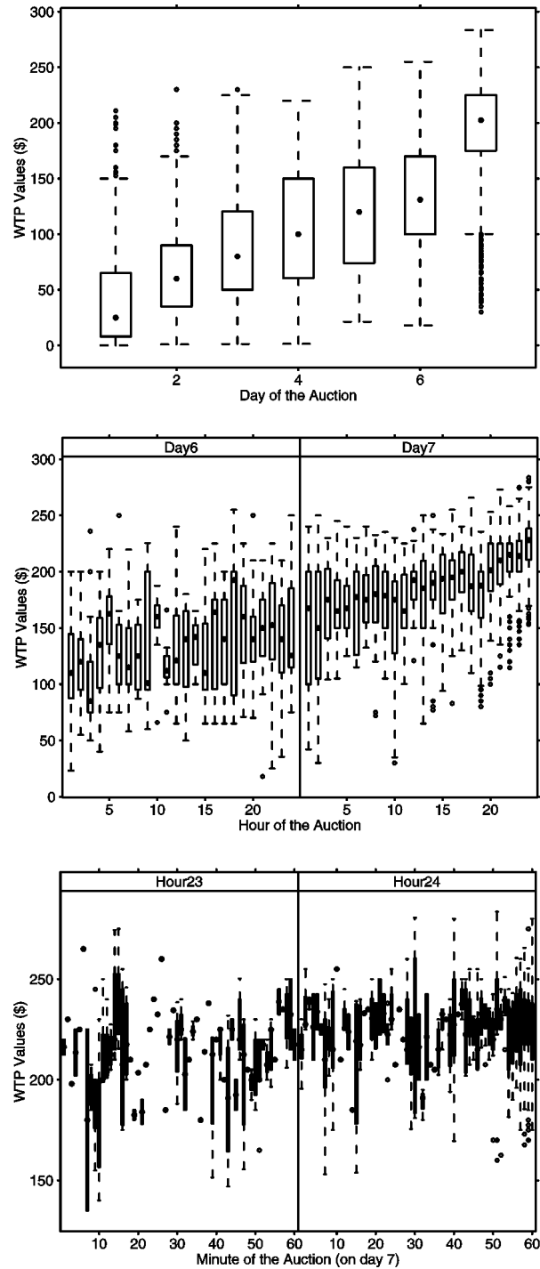
Figure 8. Illustration of STAT-zoom , by aggregating bids from 158 Palm M515 auctions at three time scales: Daily boxplots of WTP values (top), hourly boxplots for the last two days (middle), and minutely boxplots for the last two hours (bottom).
